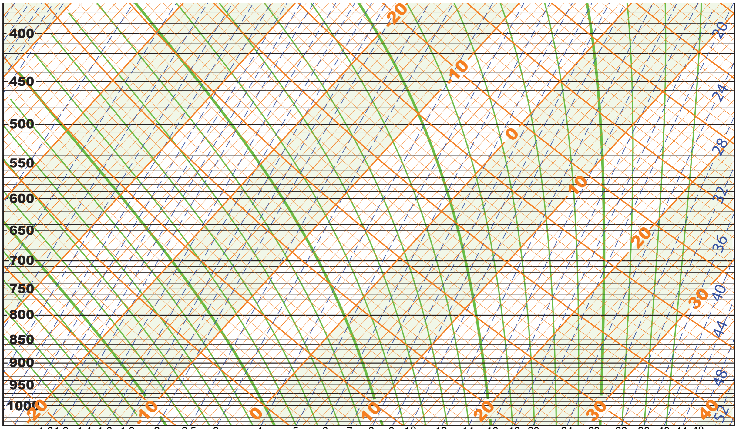
Skew-T / log p diagram for use with A First Course in Atmospheric Thermodynamics ©2008 by G.W. Petty www.sundogpublishing.com
