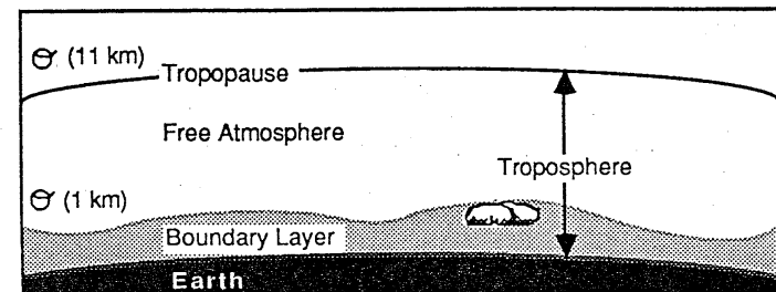
Fig. 1.1 The troposphere can be divided into two parts: a boundary layer (shaded) near the surface and the free atmosphere above it.
