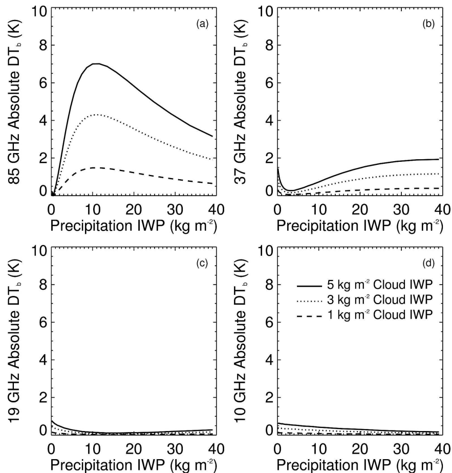
FIG. 2. Simulated absolute values of uncertainties of (a) 85-, (b) 37-, (c) 19-, and (d) 10-GHz nadir brightness temperatures ( DT_{bs} ) resulting from the existence of 1, 3, 5 \text{kg m}^{-2} cloud IWP.
