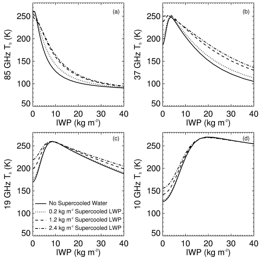
FIG. 5. Simulated nadir view brightness temperatures at (a) 85, (b) 37, (c) 19, and (d) 10 GHz as a function of IWP for supercooled LWP of 0, 0.2, 1.2, and 2.4 \text{kg m}^{-2} .
