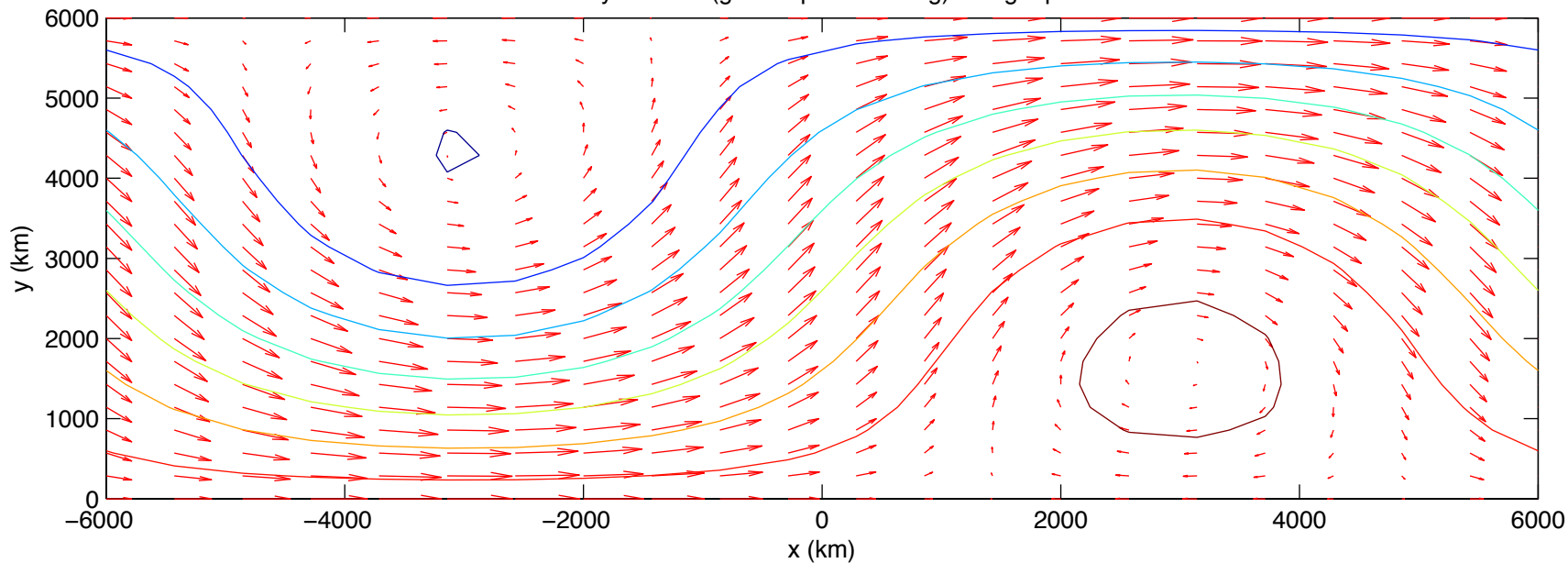
mixed layer winds (geostrophic: no drag) and geopotential
