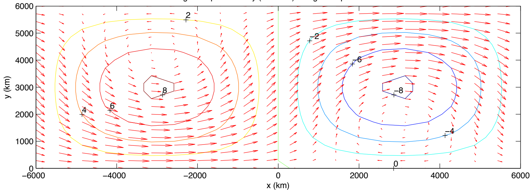
geostrophic vorticity ( 10^{-6} \text{ s}^{-1} ) and geostrophic wind
