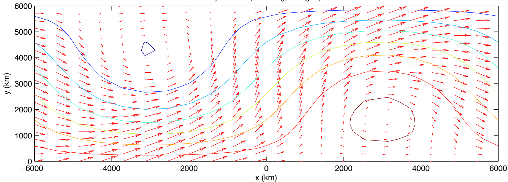
mixed layer winds (with drag) and geopotential
