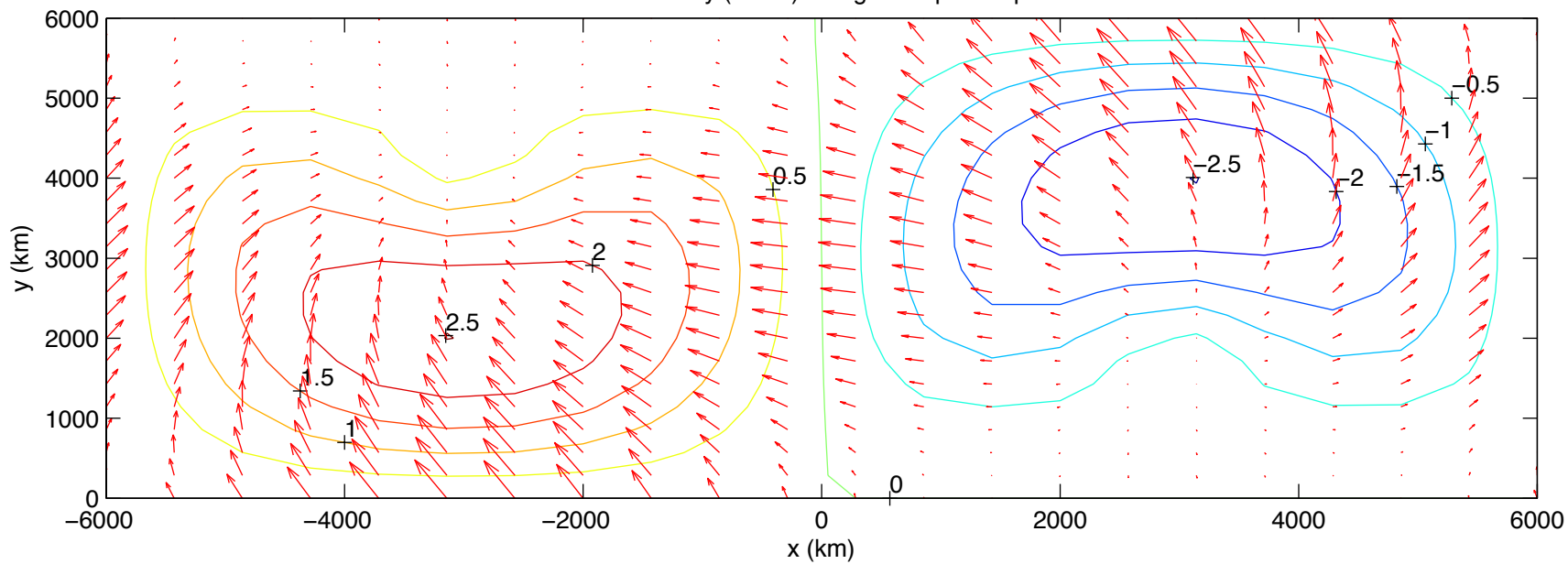
vertical velocity (mm/s) and geostrophic departure
