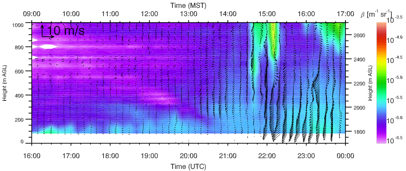
LiDAR Backscatter and VAD winds
