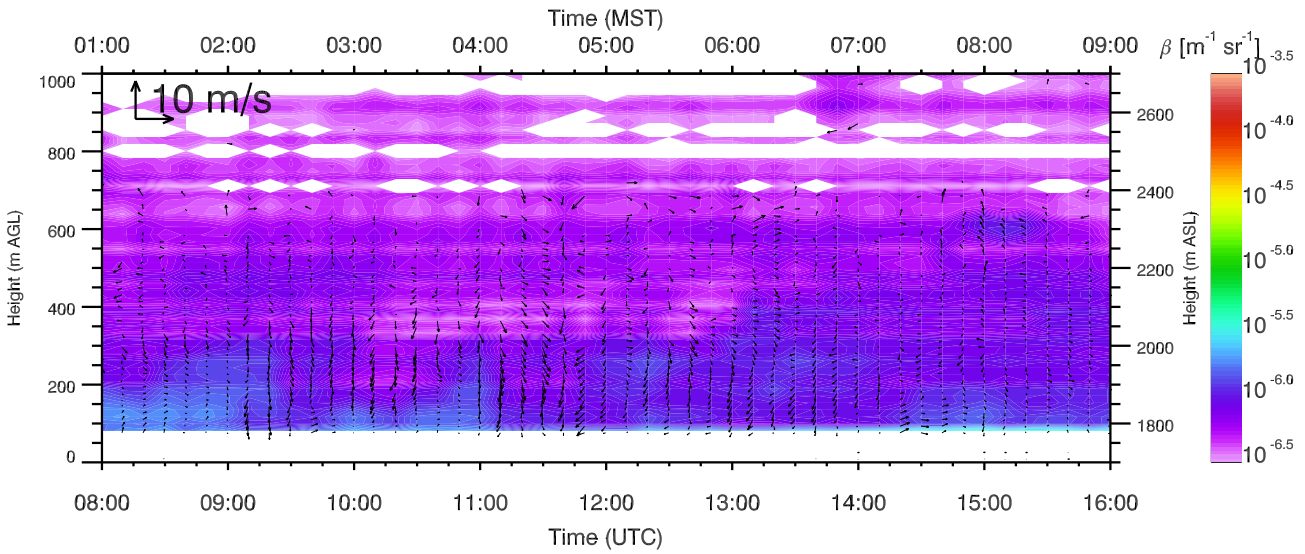
LiDAR Backscatter and VAD winds
