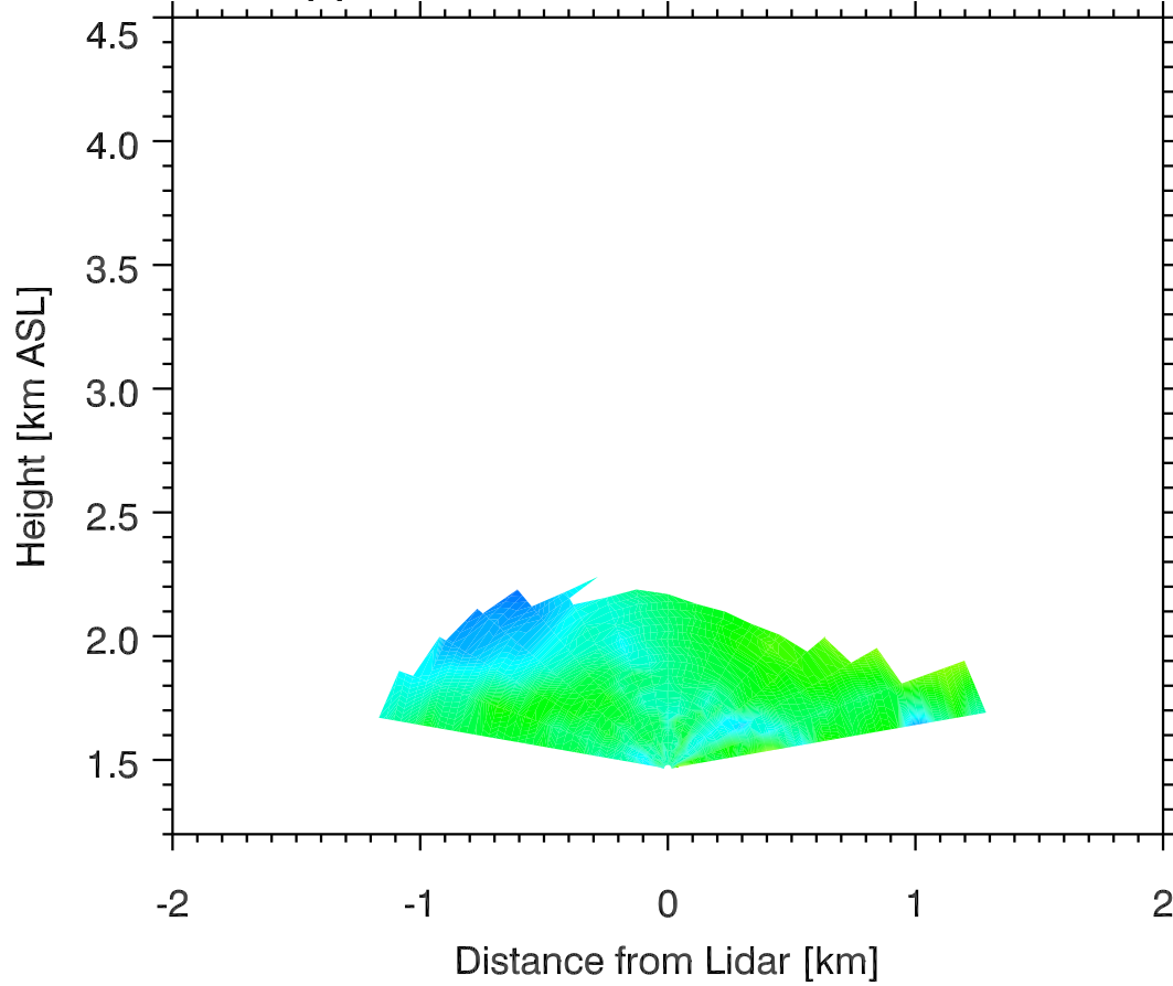
Doppler Winds 05 Nov 2011 0613 MST
