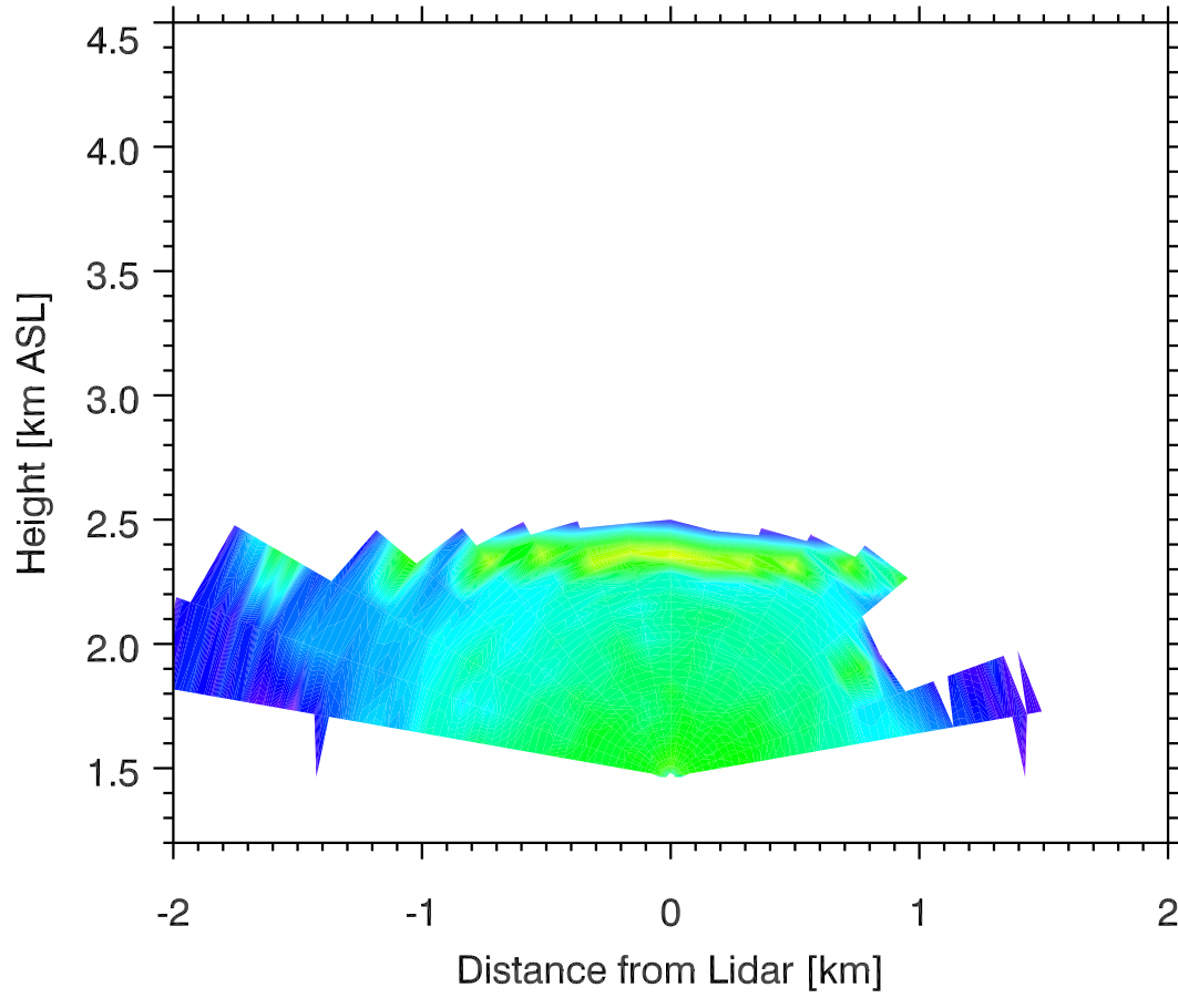
Backscatter 05 Nov 2011 0443 MST
