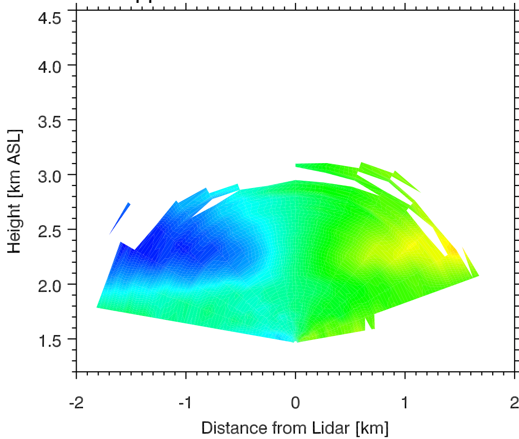
Doppler Winds 05 Nov 2011 0349 MST
