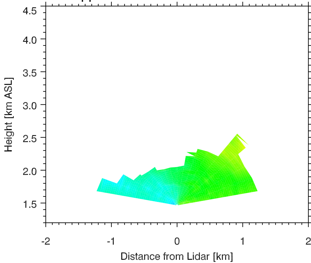
Doppler Winds 05 Nov 2011 0407 MST
