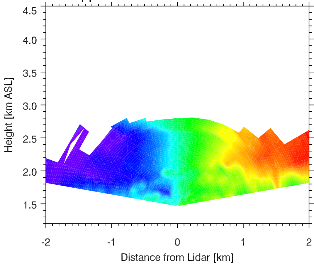
Doppler Winds 05 Nov 2011 0501 MST
