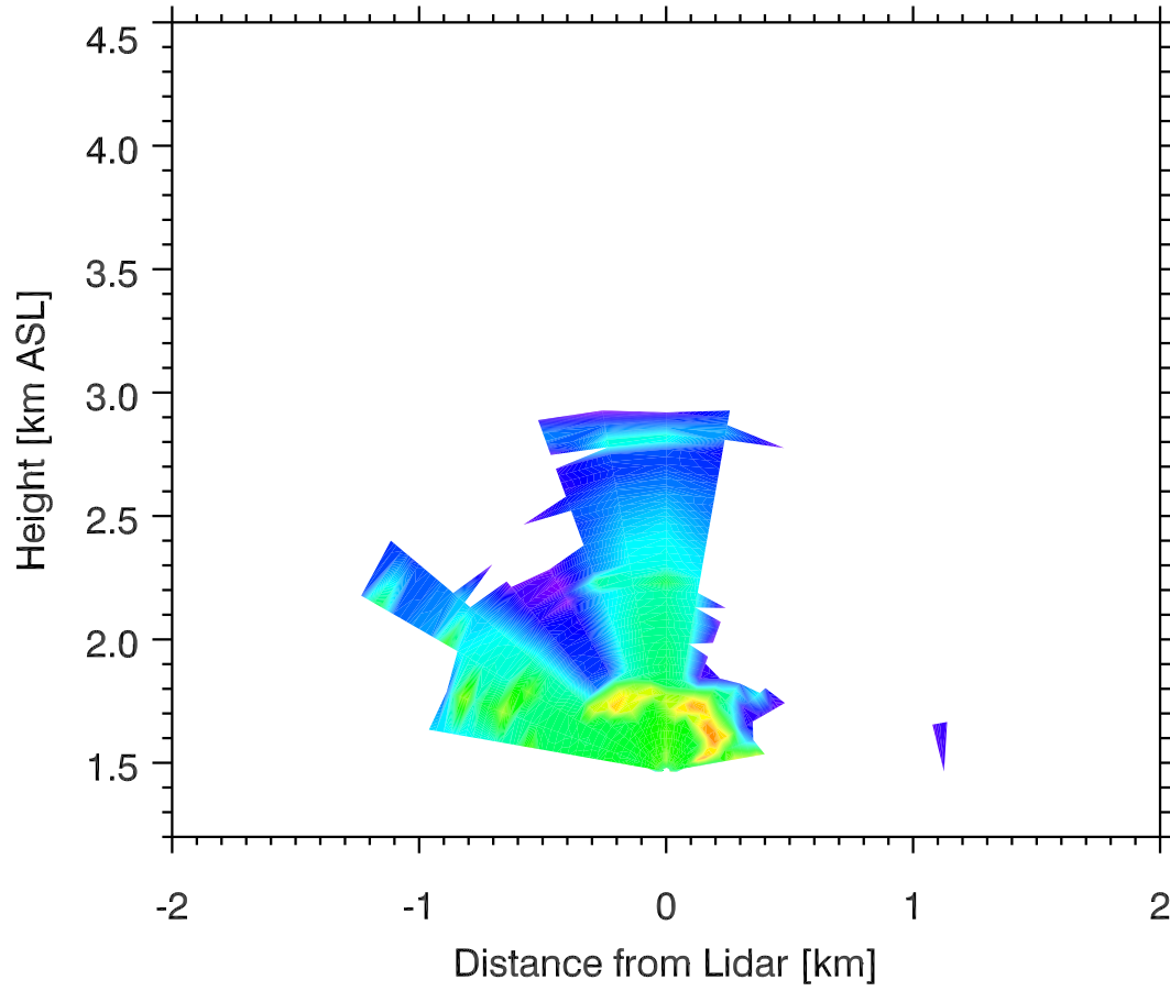
Backscatter 05 Nov 2011 0355 MST
