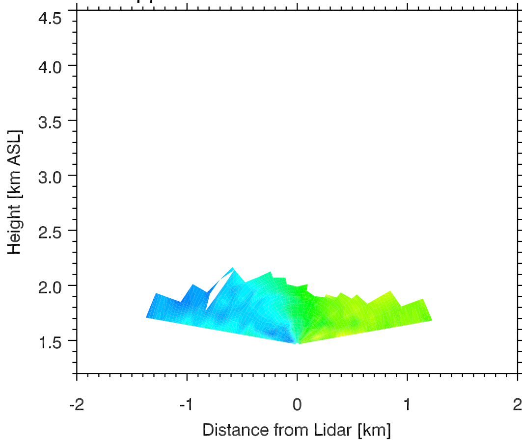
Doppler Winds 05 Nov 2011 0425 MST
