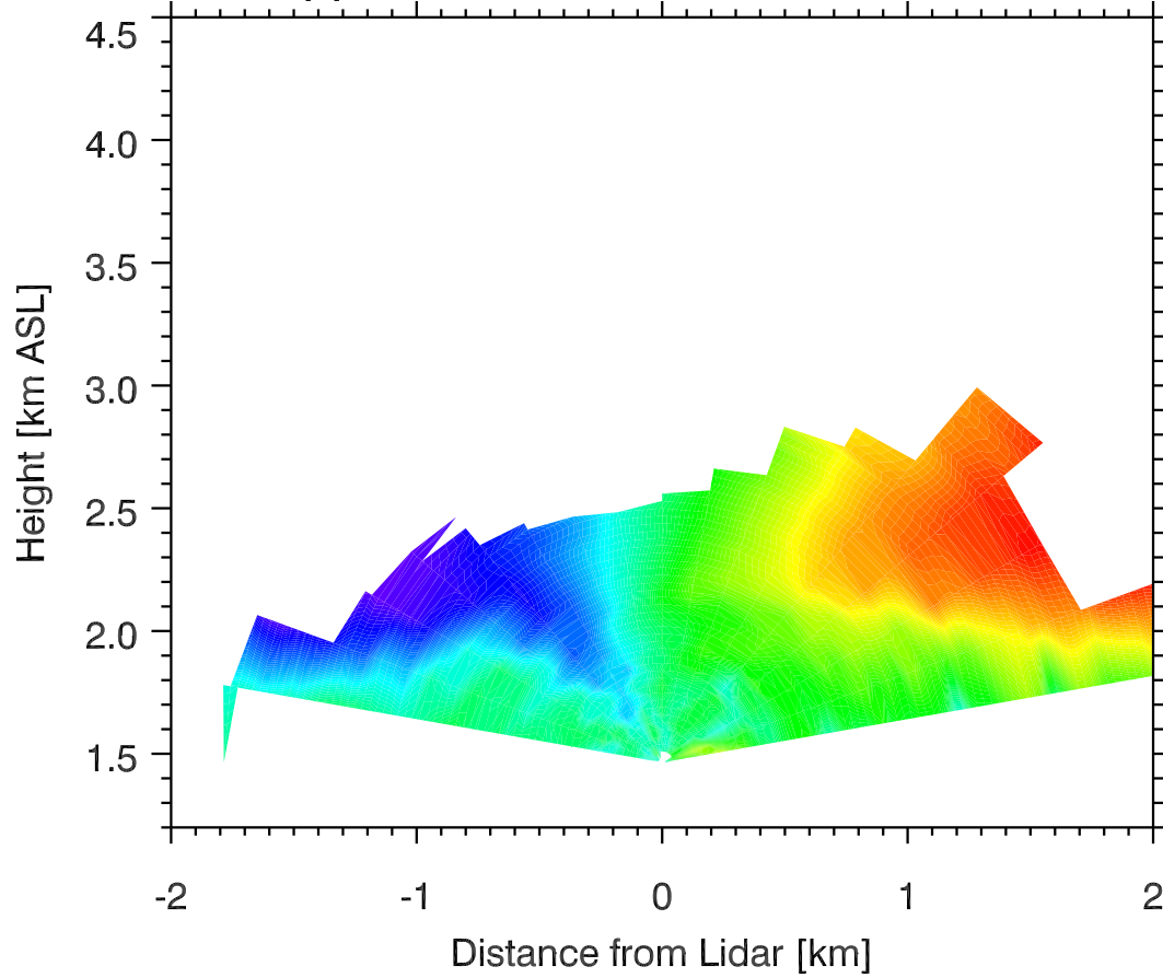
Doppler Winds 05 Nov 2011 0601 MST
