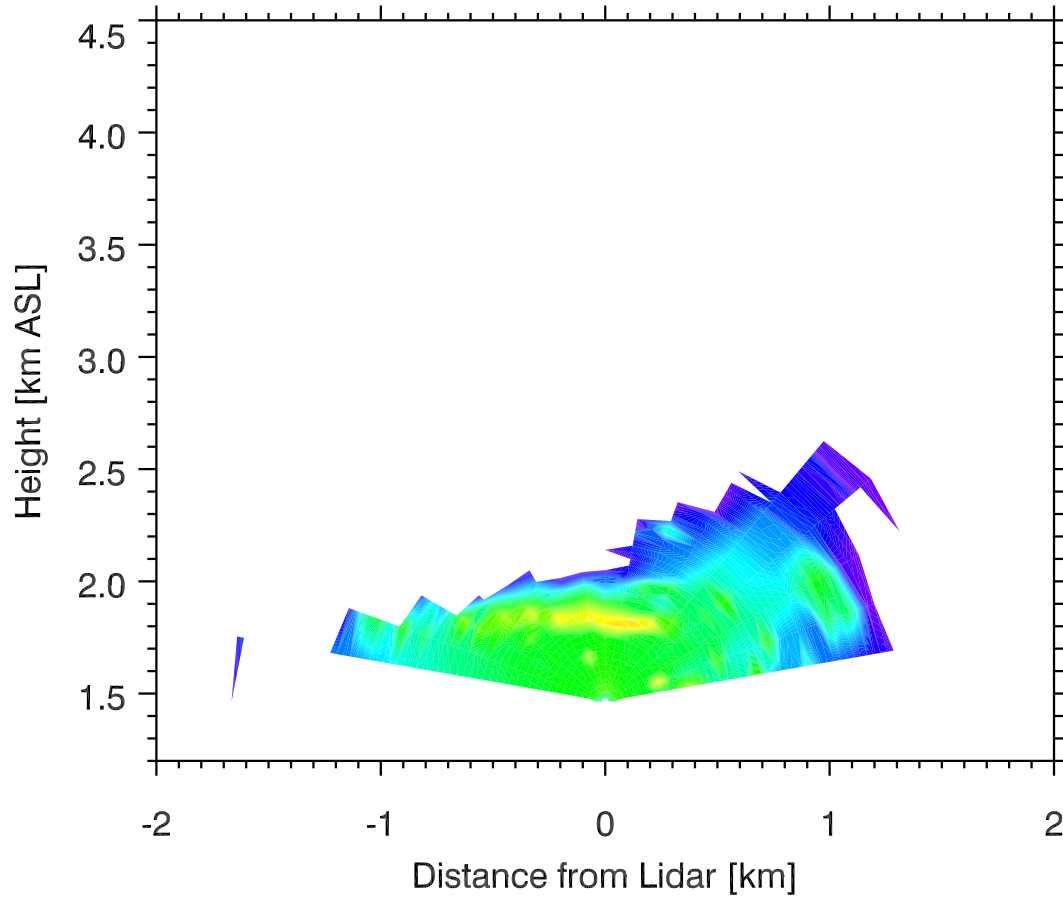
Backscatter 05 Nov 2011 0407 MST
