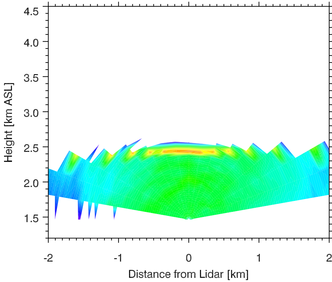
Backscatter 05 Nov 2011 0531 MST
