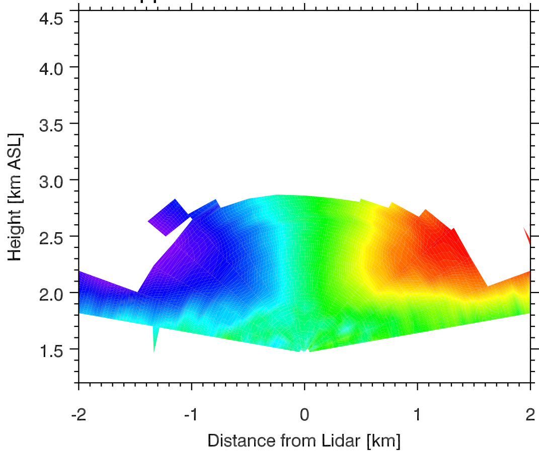
Doppler Winds 05 Nov 2011 0555 MST
