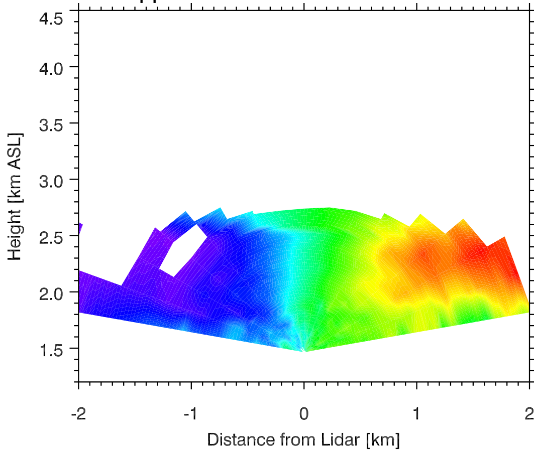
Doppler Winds 05 Nov 2011 0455 MST
