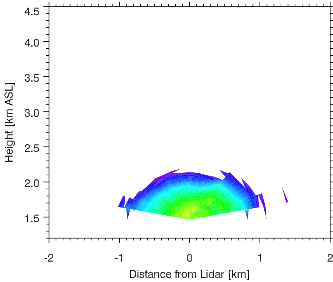
Backscatter 05 Nov 2011 0619 MST
