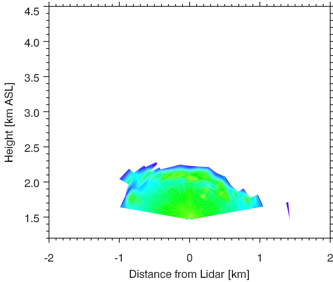
Backscatter 05 Nov 2011 0437 MST
