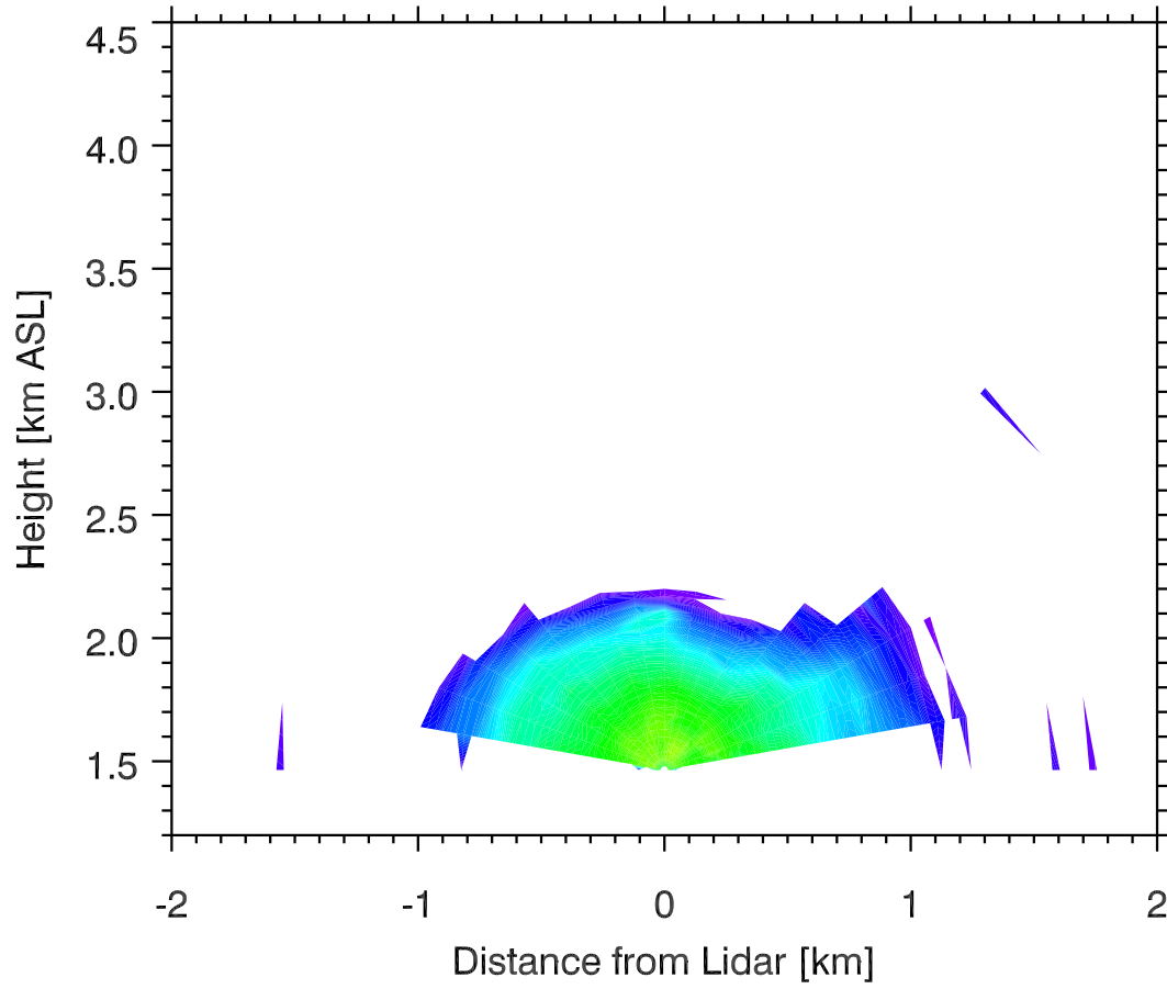
Backscatter 05 Nov 2011 0625 MST
