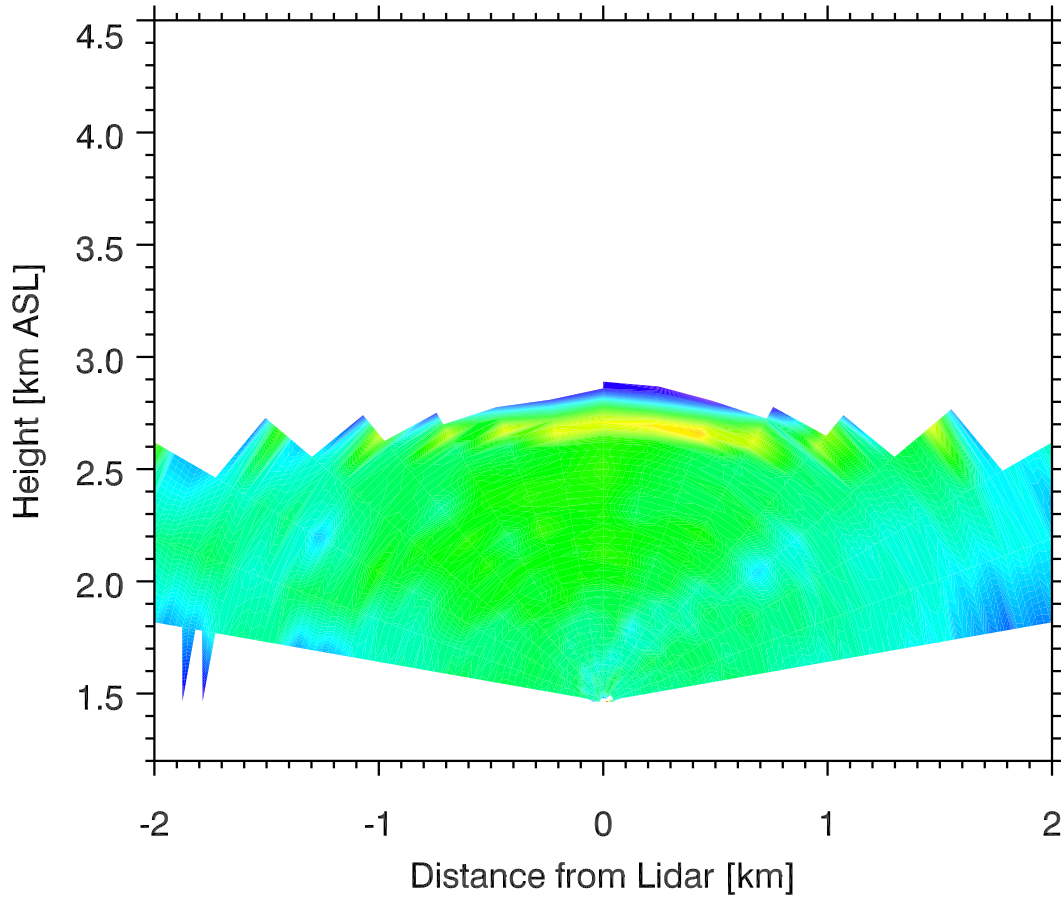
Backscatter 05 Nov 2011 0549 MST
