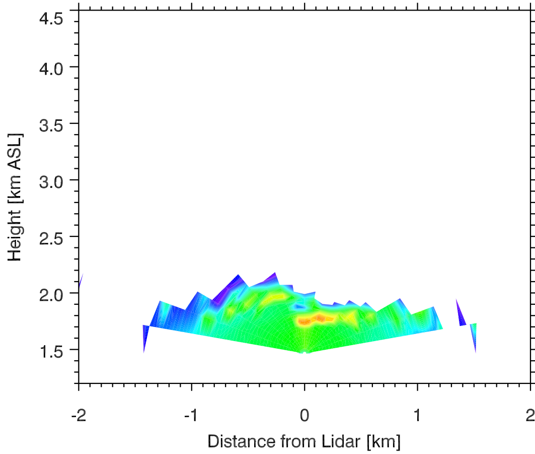
Backscatter 05 Nov 2011 0425 MST
