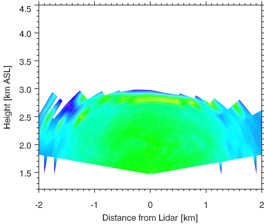
Backscatter 05 Nov 2011 0513 MST
