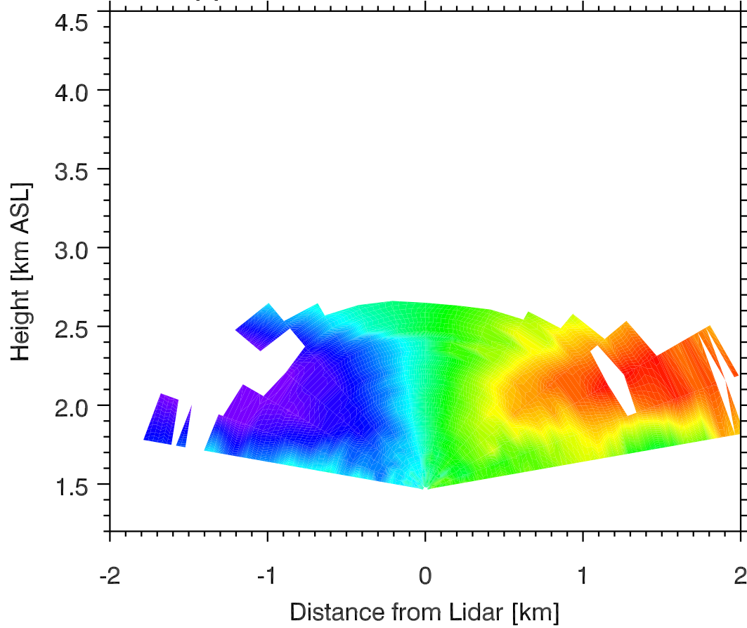
Doppler Winds 05 Nov 2011 0449 MST
