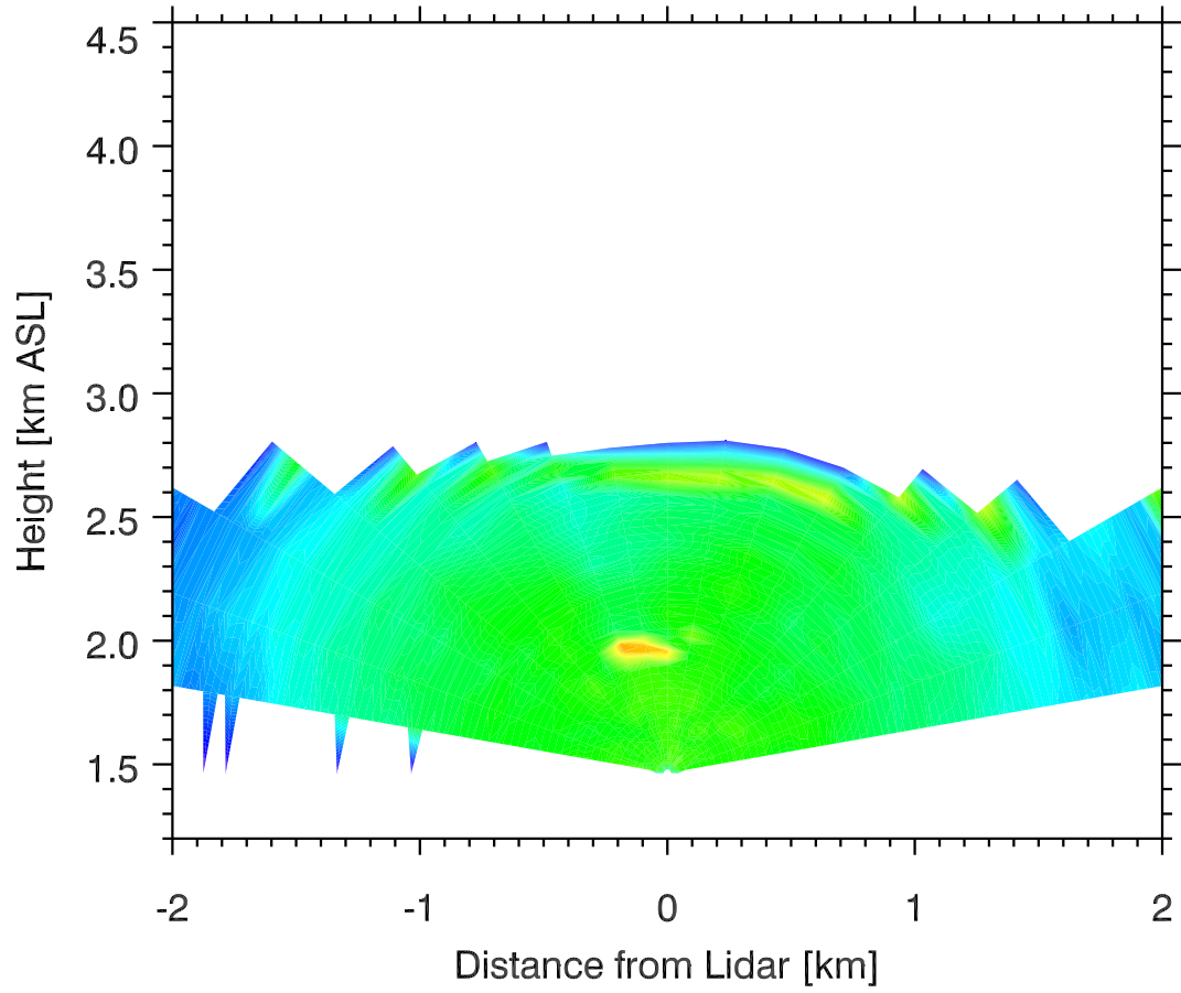
Backscatter 05 Nov 2011 0501 MST
