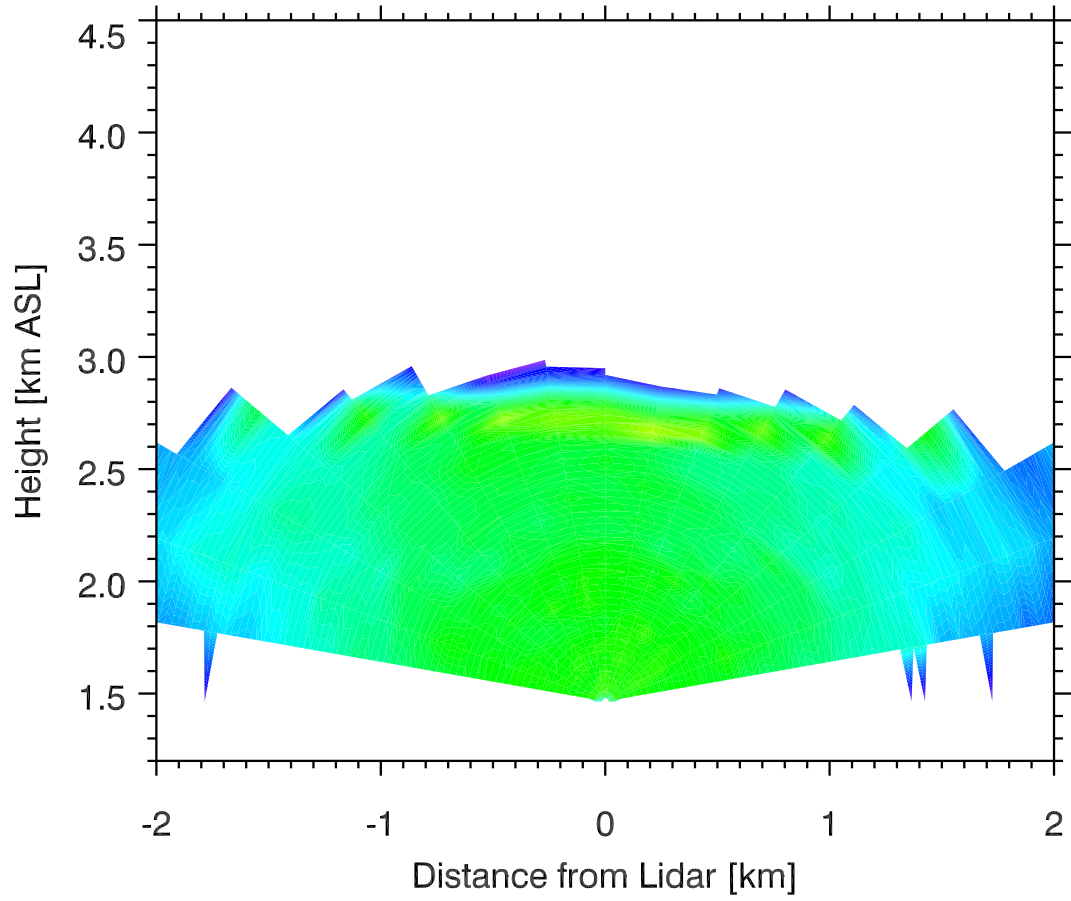
Backscatter 05 Nov 2011 0507 MST
