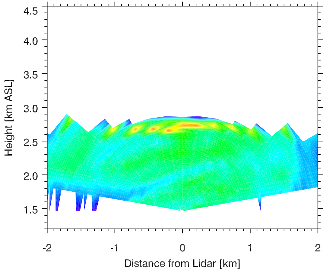
Backscatter 05 Nov 2011 0555 MST
