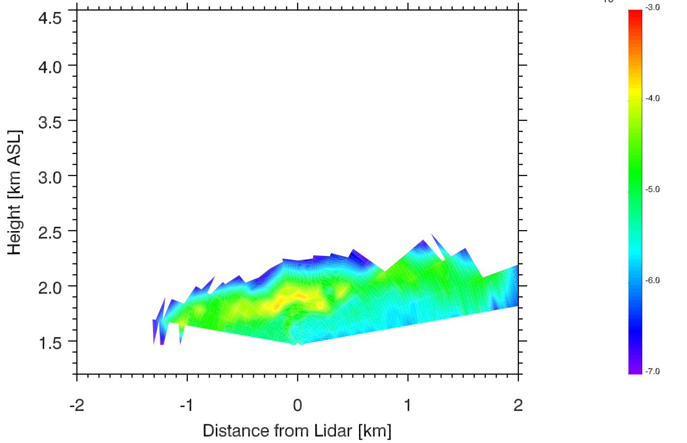
Backscatter 05 Nov 2011 0607 MST
