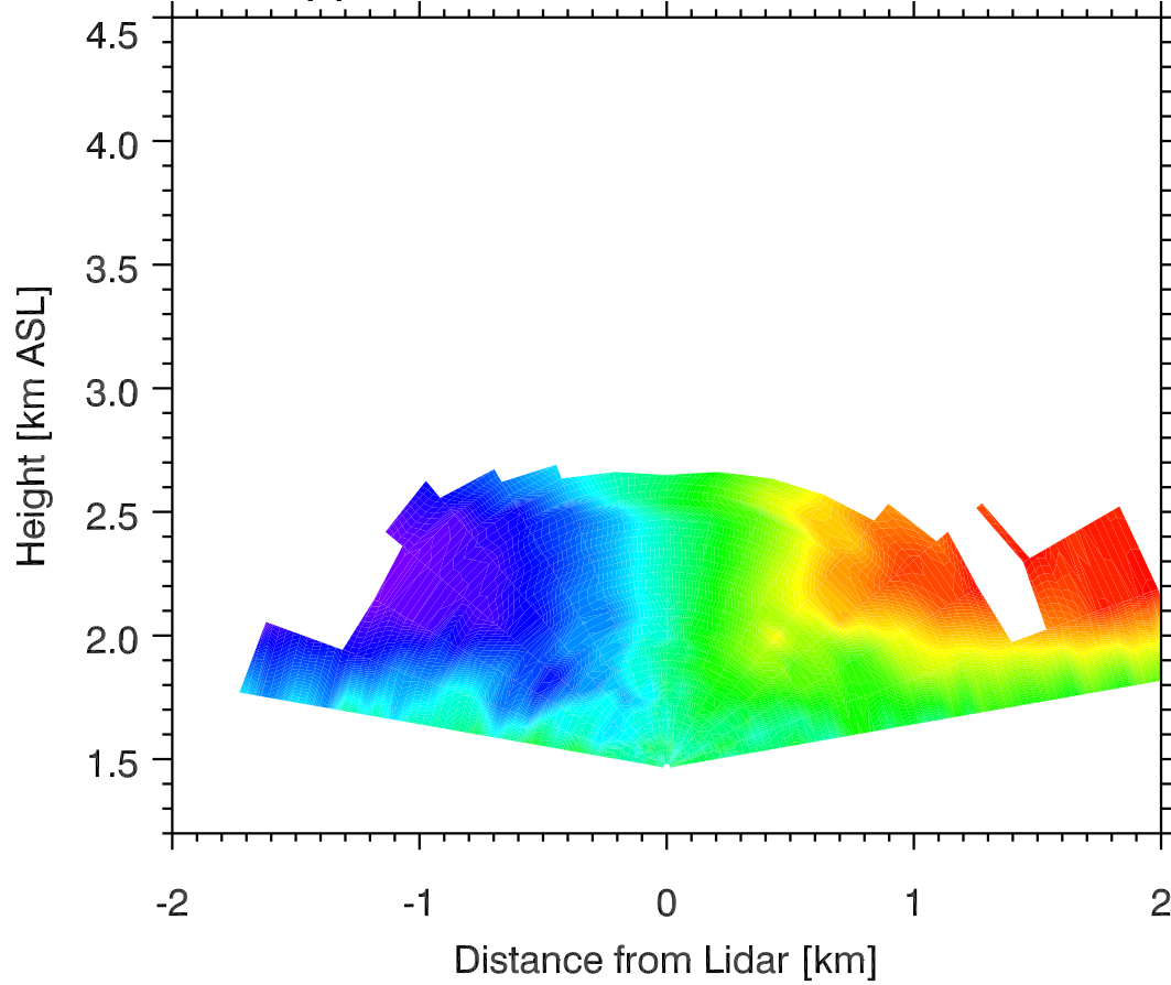
Doppler Winds 05 Nov 2011 0537 MST
