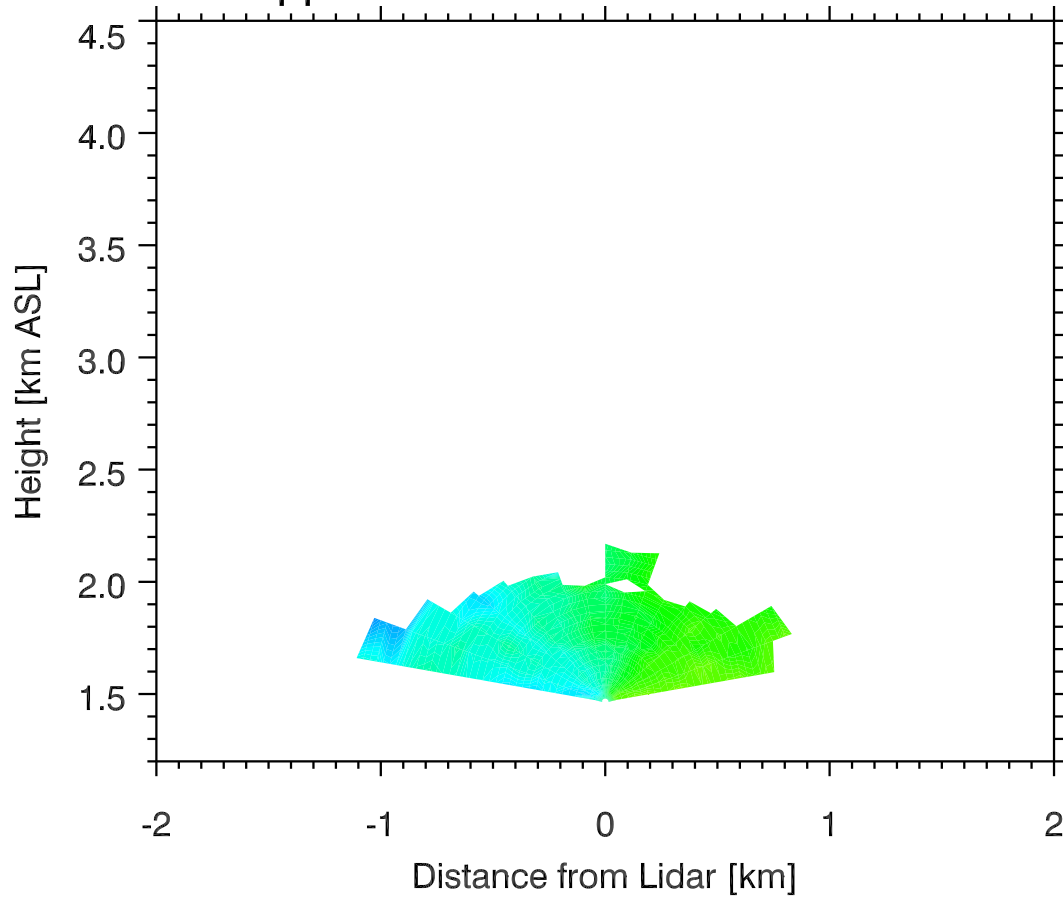
Doppler Winds 05 Nov 2011 0413 MST
