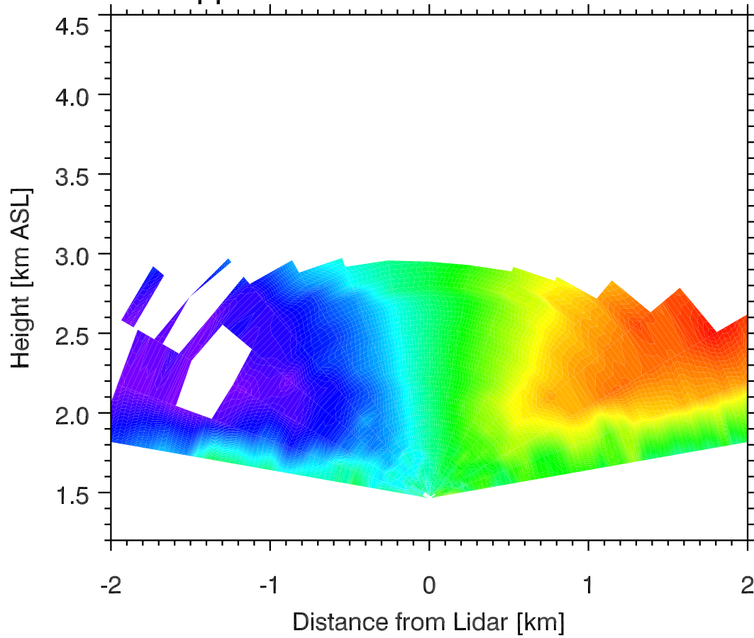
Doppler Winds 05 Nov 2011 0513 MST
