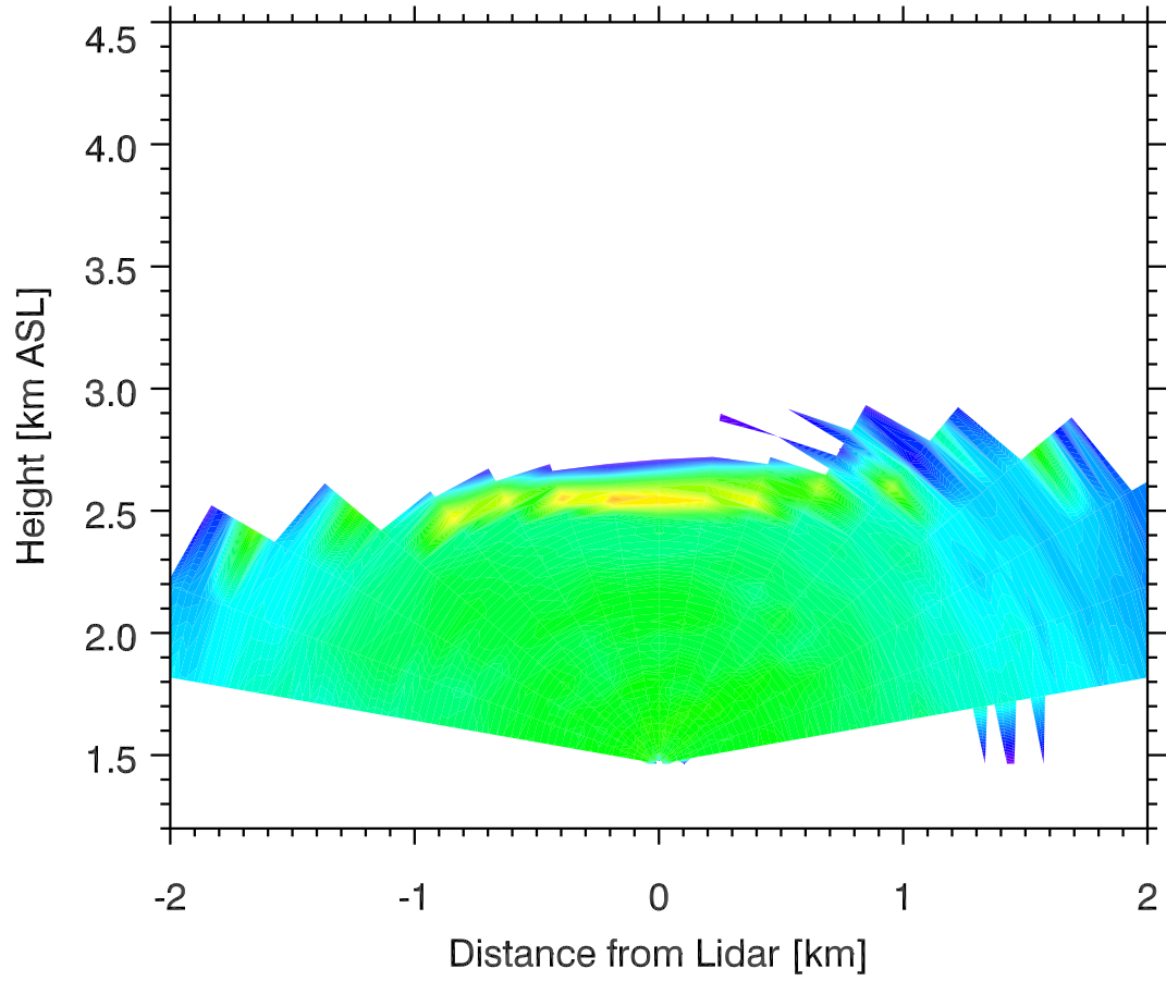
Backscatter 05 Nov 2011 0519 MST
