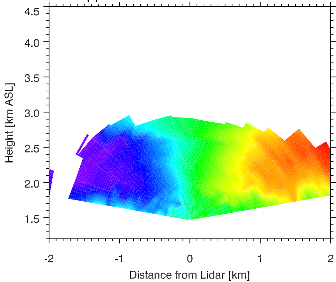
Doppler Winds 05 Nov 2011 0507 MST
