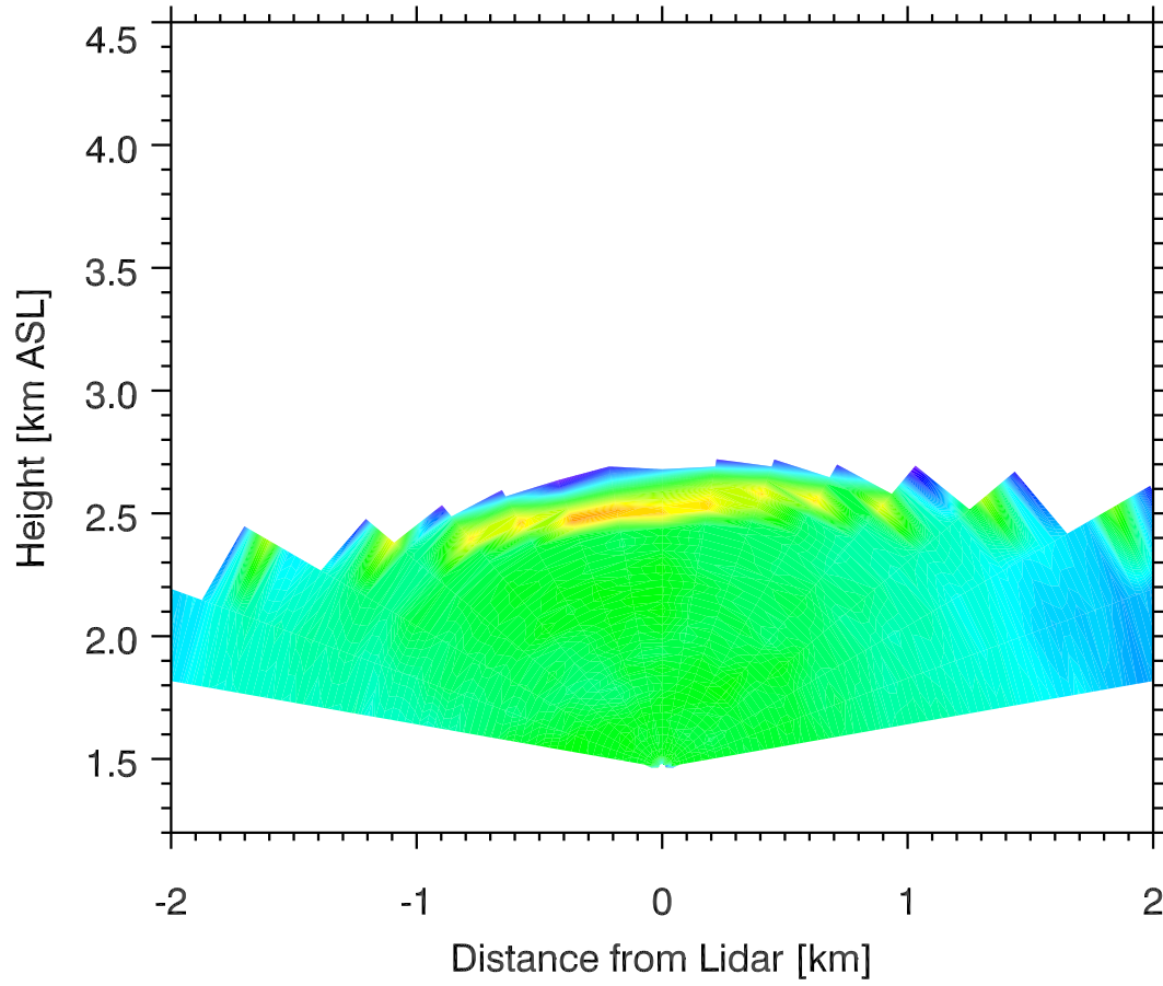
Backscatter 05 Nov 2011 0525 MST
