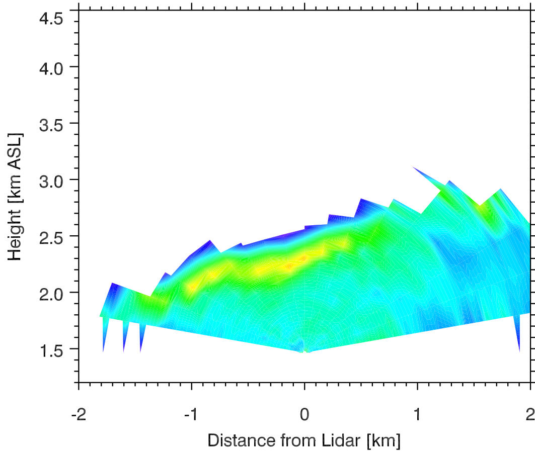
Backscatter 05 Nov 2011 0601 MST
