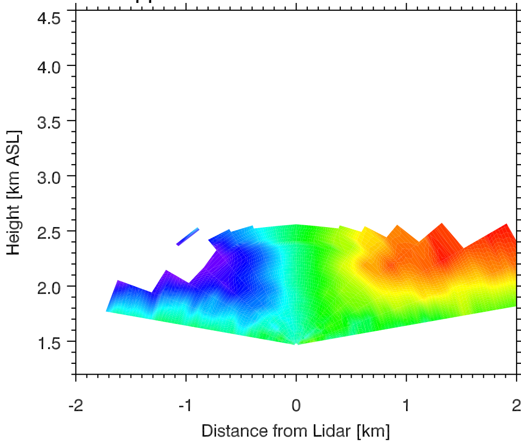
Doppler Winds 05 Nov 2011 0531 MST
