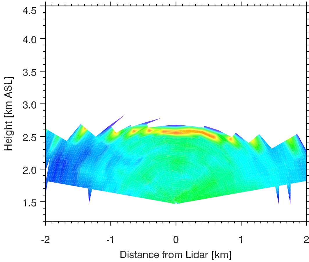
Backscatter 05 Nov 2011 0537 MST
