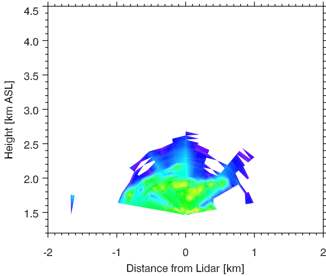
Backscatter 05 Nov 2011 0401 MST
