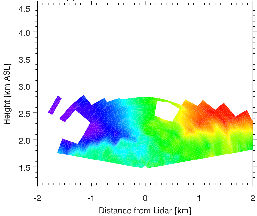
Doppler Winds 05 Nov 2011 0543 MST
