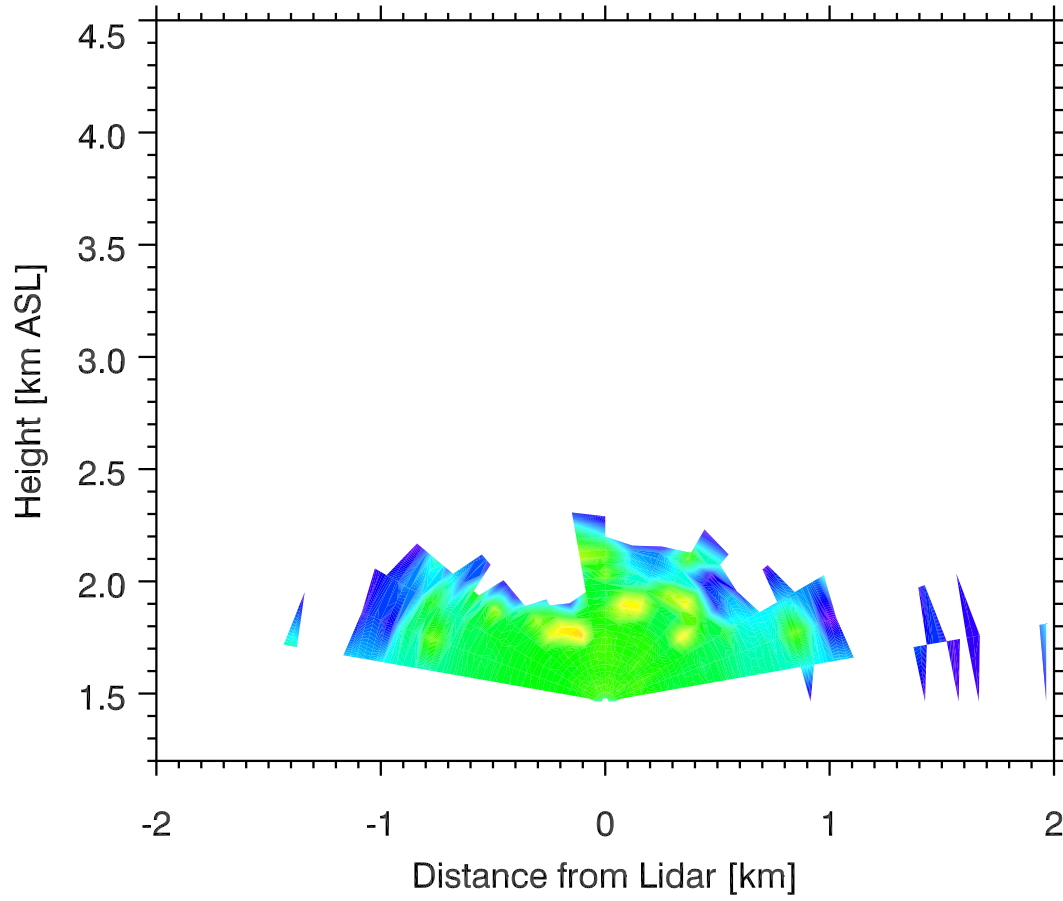
Backscatter 05 Nov 2011 0431 MST
