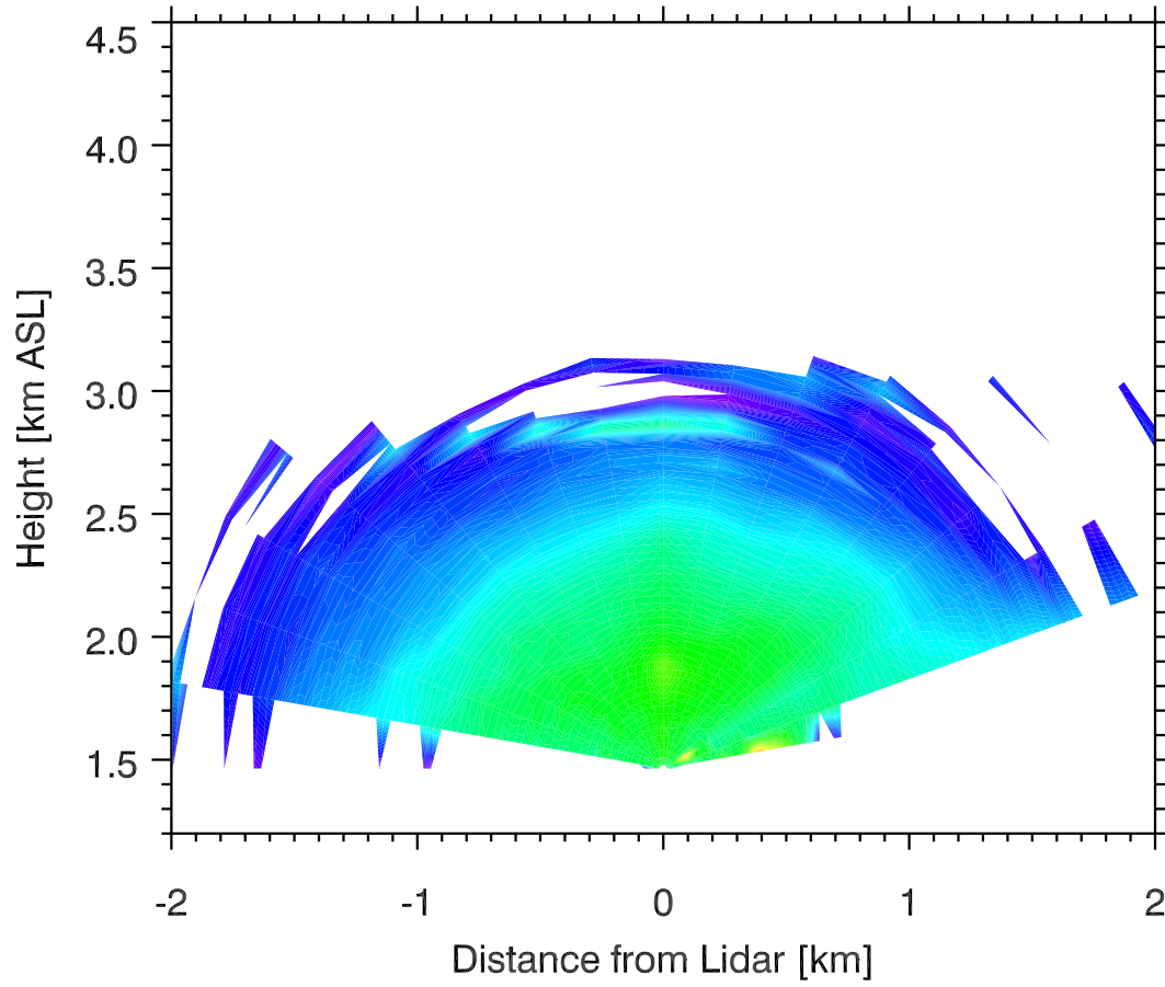
Backscatter 05 Nov 2011 0349 MST
