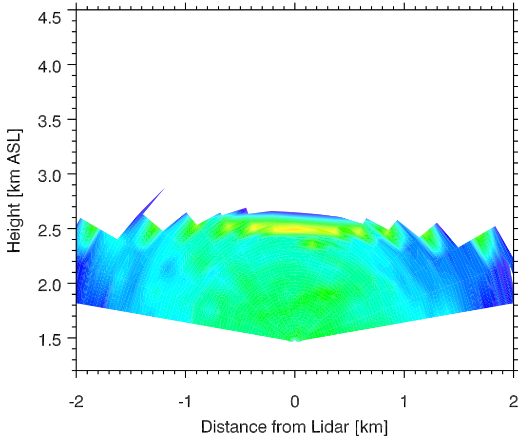
Backscatter 05 Nov 2011 0449 MST
