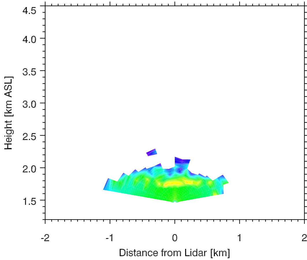
Backscatter 05 Nov 2011 0413 MST
