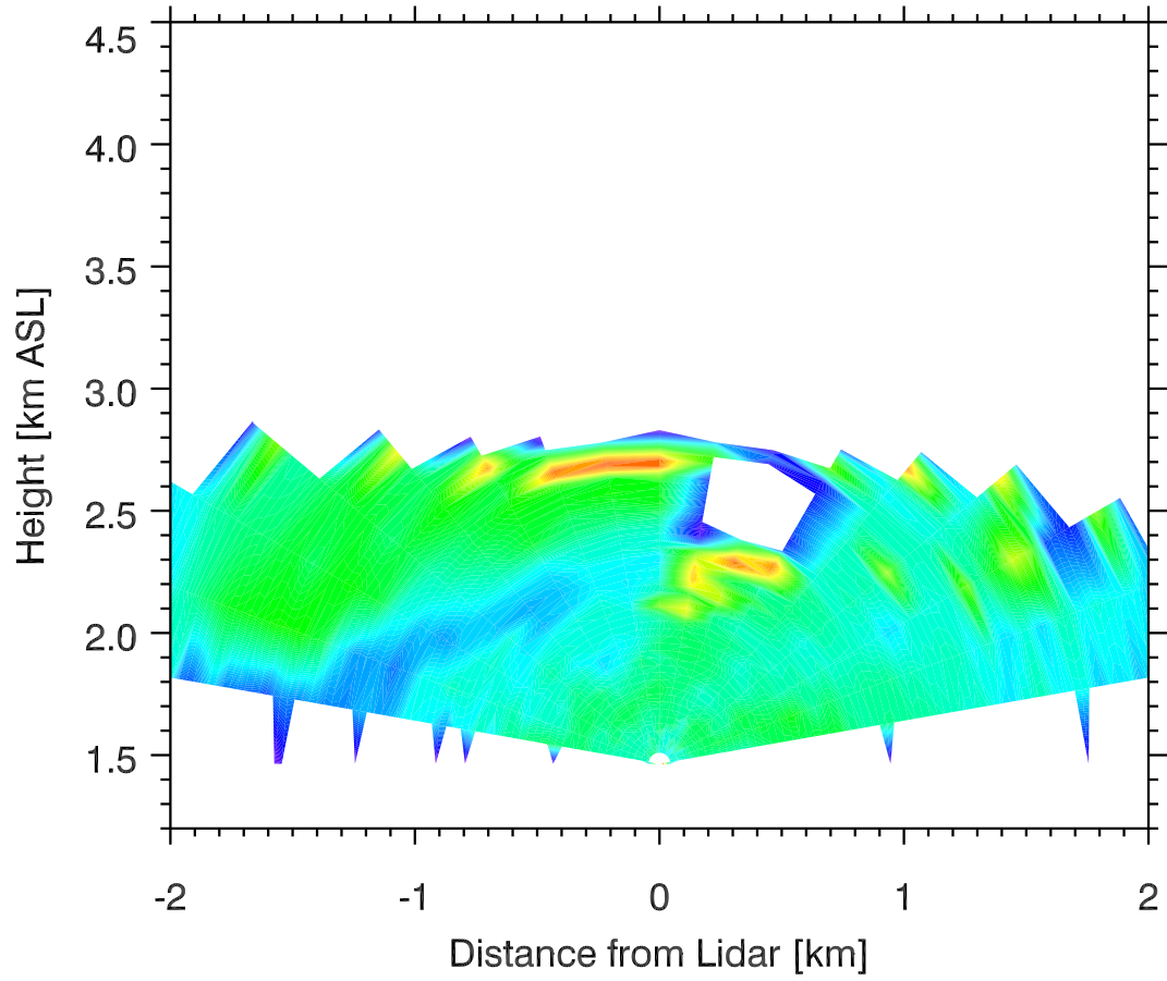
Backscatter 05 Nov 2011 0543 MST
