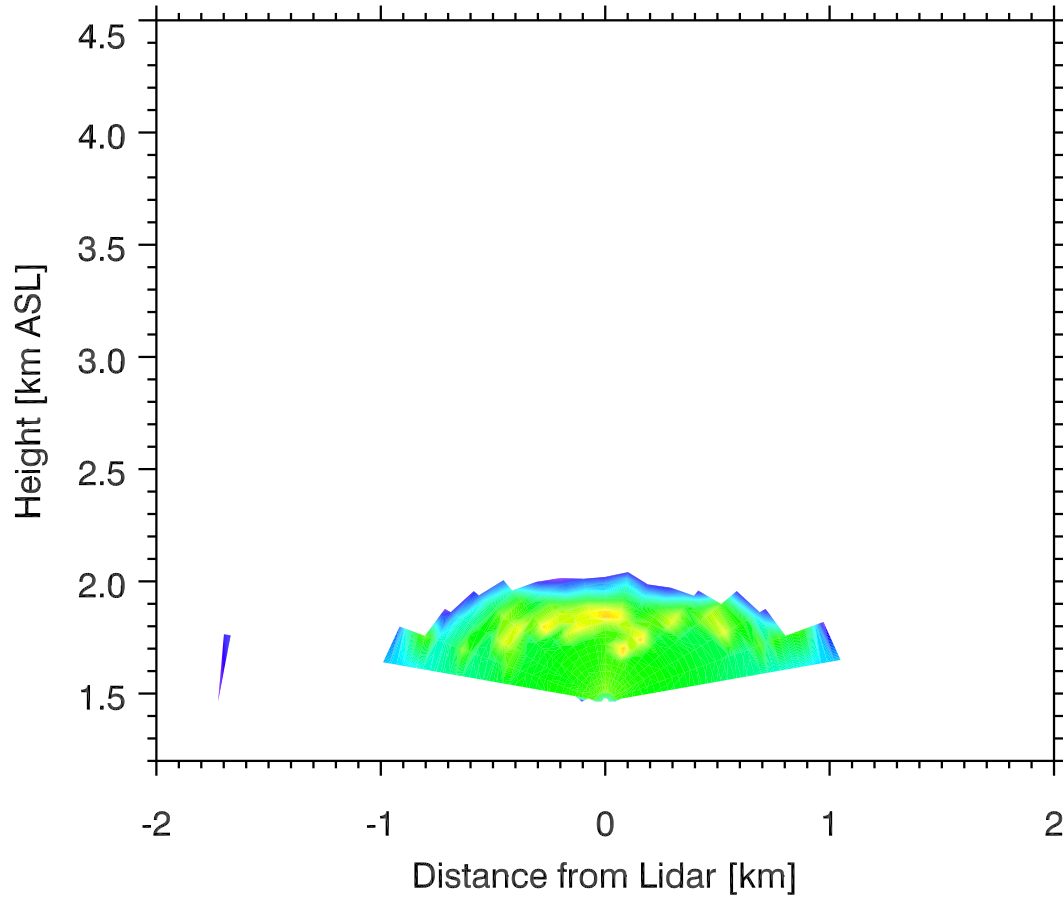
Backscatter 05 Nov 2011 0419 MST
