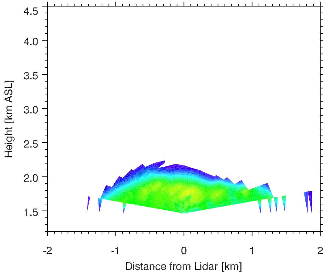
Backscatter 05 Nov 2011 0613 MST
