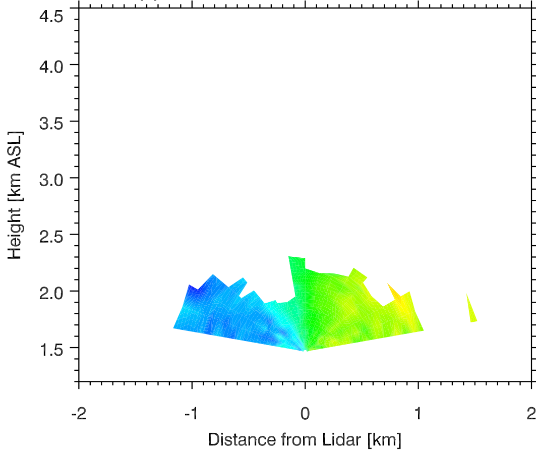
Doppler Winds 05 Nov 2011 0431 MST
