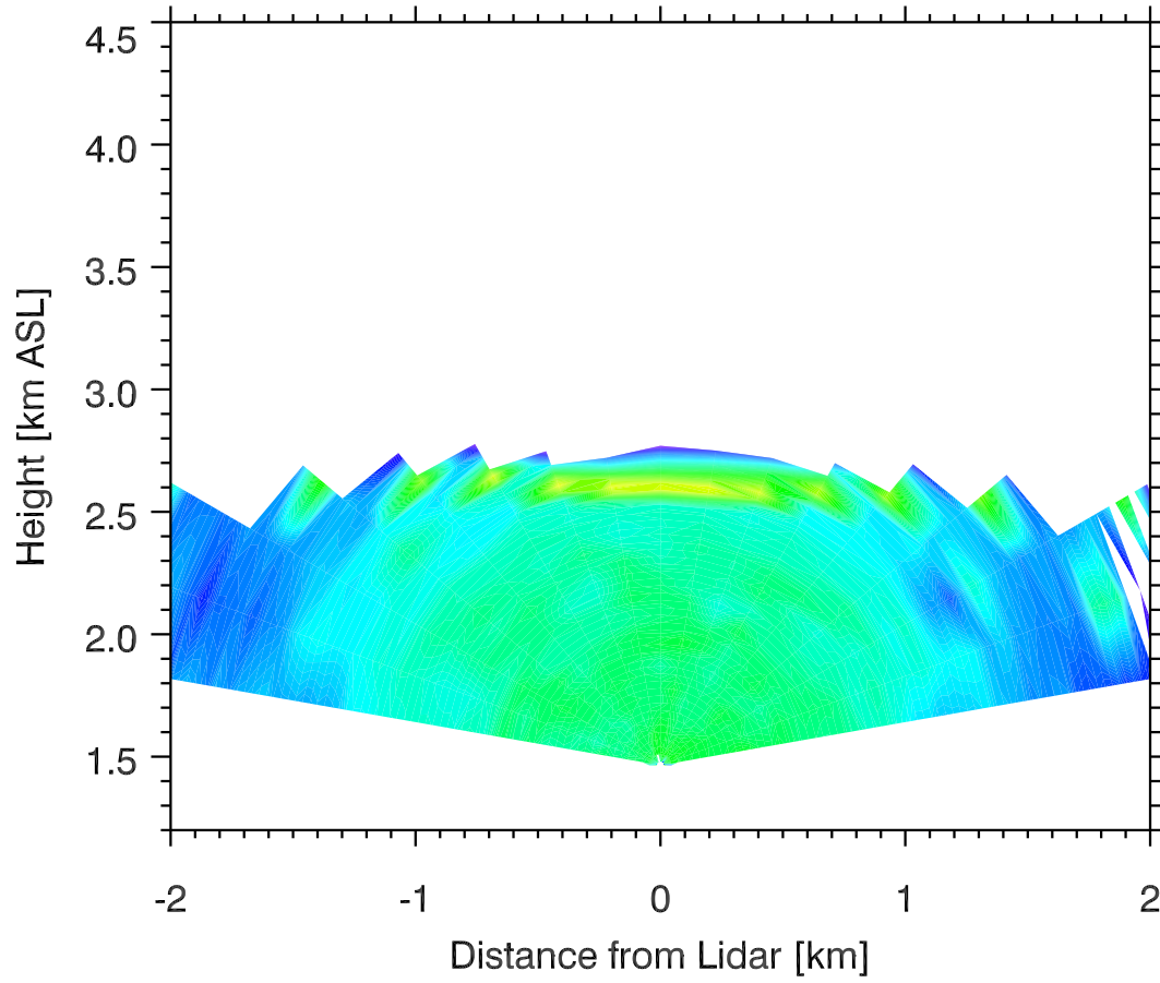
Backscatter 05 Nov 2011 0455 MST
