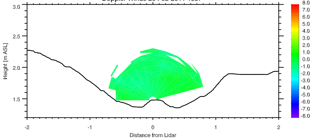
Doppler Winds 26 Feb 2011 1337
