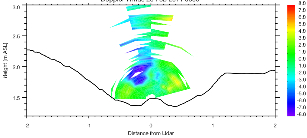
Doppler Winds 26 Feb 2011 0000
