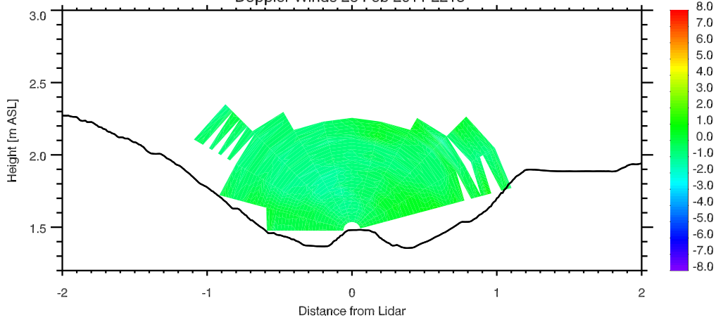
Doppler Winds 26 Feb 2011 2213
