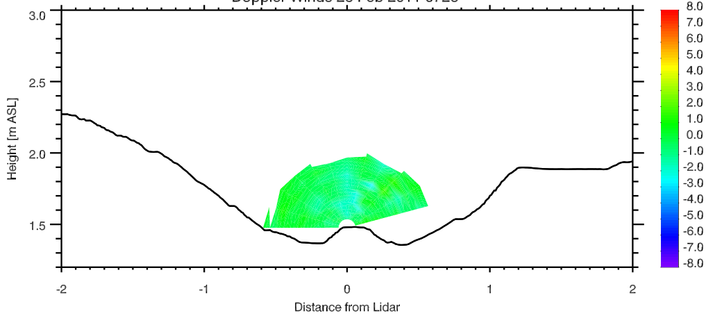
Doppler Winds 26 Feb 2011 0726
