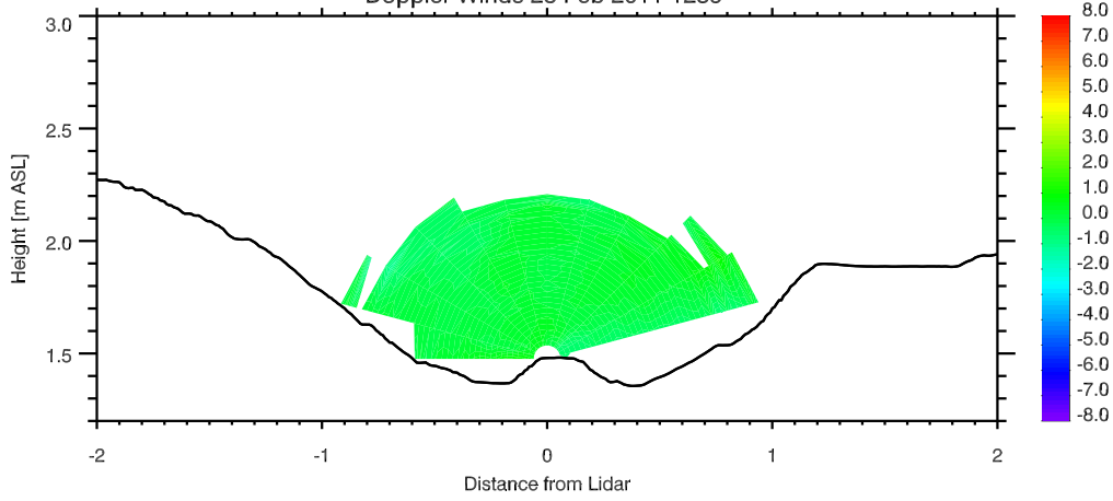
Doppler Winds 28 Feb 2011 1239
