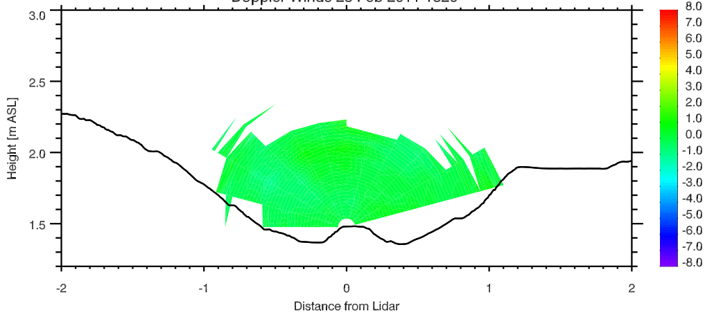
Doppler Winds 28 Feb 2011 1820
