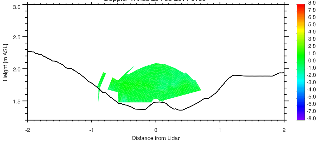
Doppler Winds 28 Feb 2011 0133
