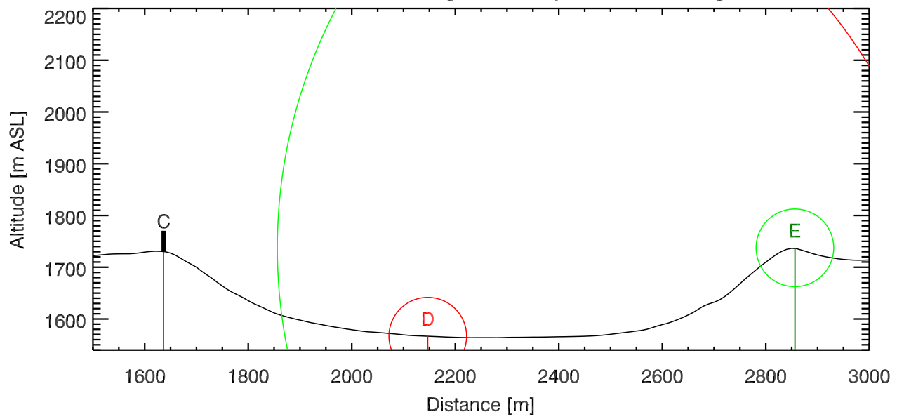
Cross section through SW-Gap, Azi.: 22.5 deg
