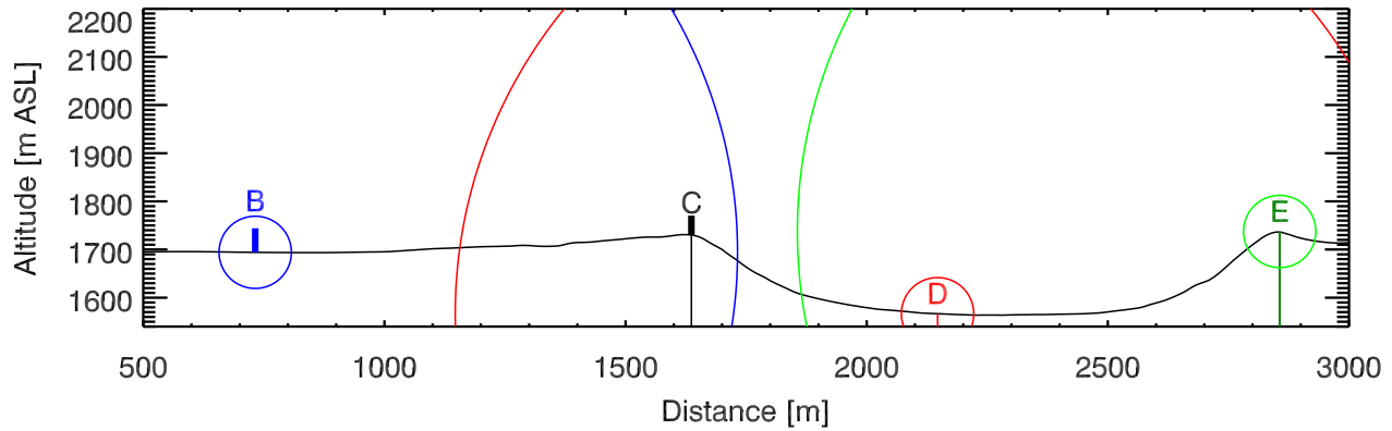
Cross section through SW-Gap, Azi.: 22.5 deg
