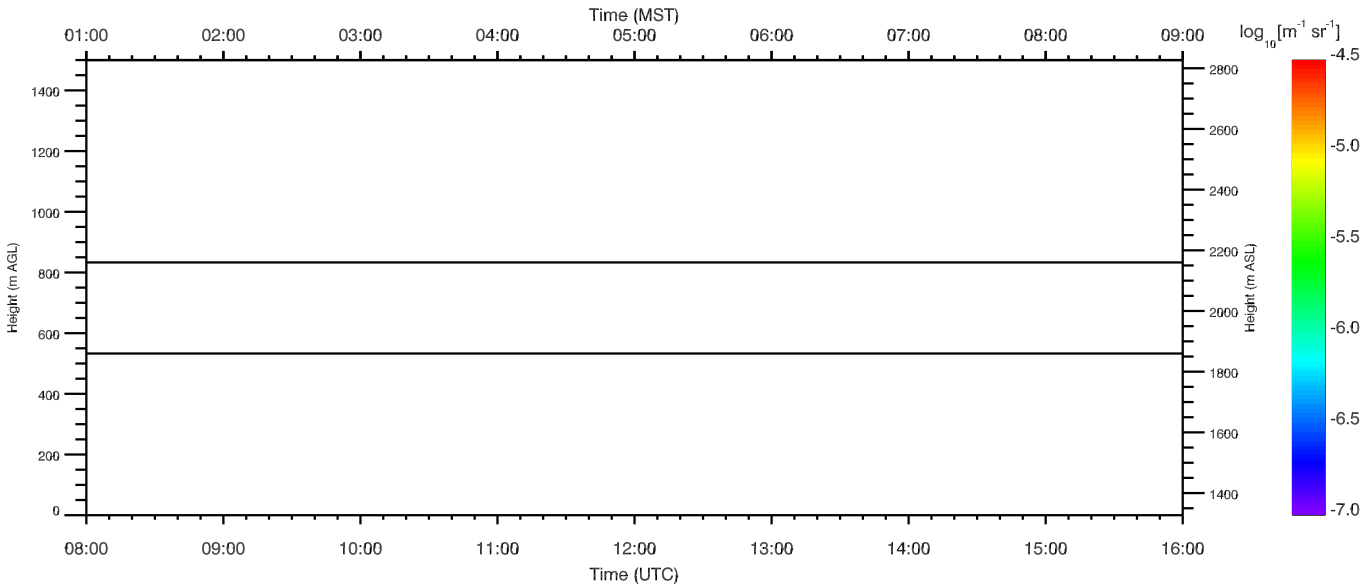
Backscatter 12 Oct 2012 0800 - 12 Oct 2012 1600
