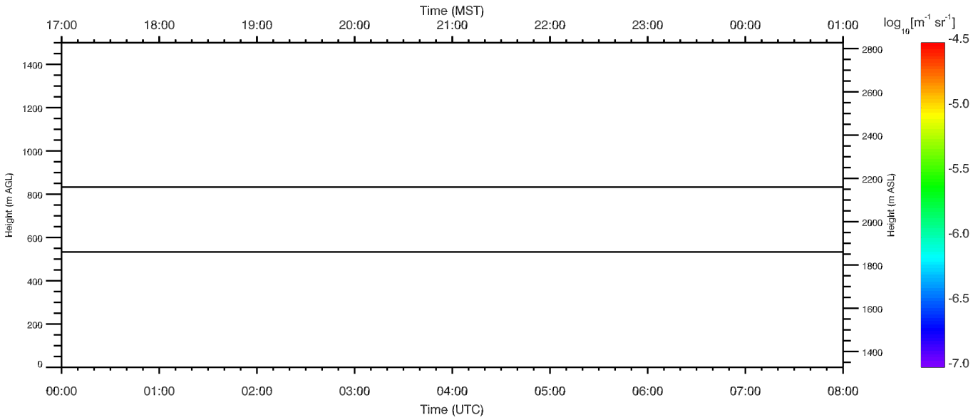
Backscatter 12 Oct 2012 0000 - 12 Oct 2012 0800
