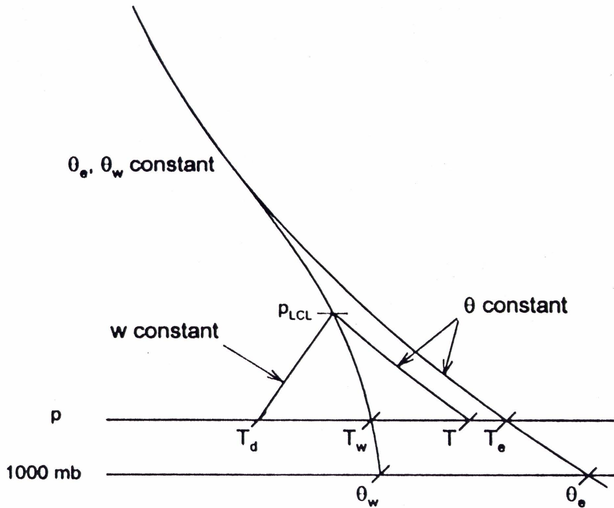
Figure 6.10 Depiction of thermodynamic variations on a skew- T diagram from which all but the essential isopleths are omitted.
