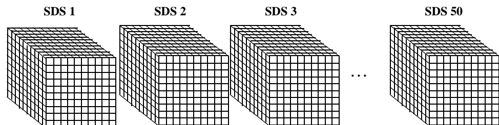
50 10 \times 10 \times 10 Element Scientific Data Sets
