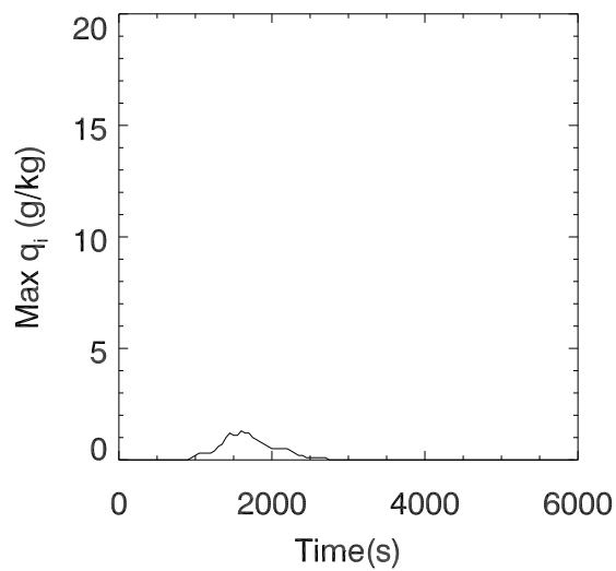
cloud ice, 15km bubble
