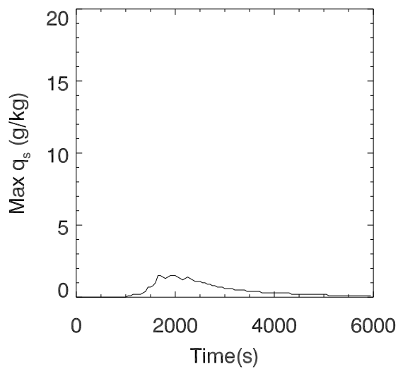
snow, 15km bubble
