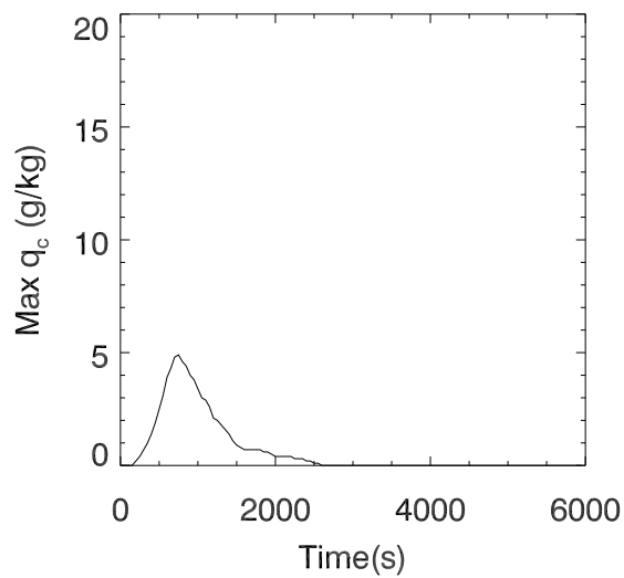
cloud water, 15km bubble
