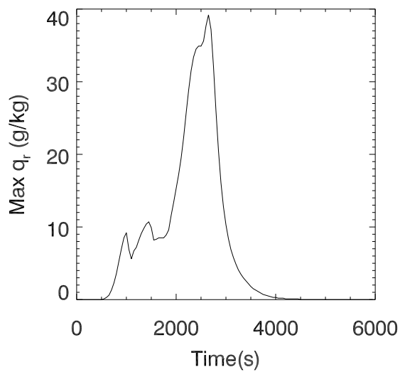
rain, 15km bubble
