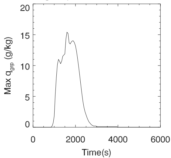
graupel, 15km bubble
