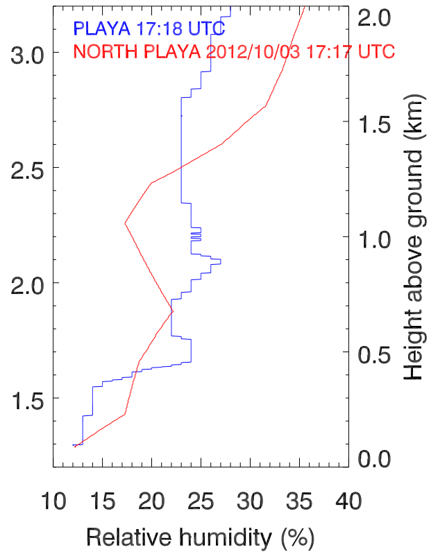
MATERHORN INTERCOMP
